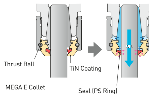
Through tools with PS ring
