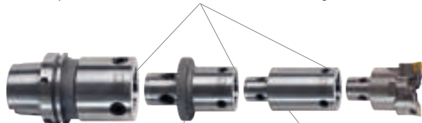
All components with recess for the CKB floating cross-bolt
