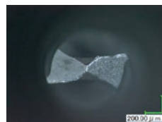
Drill tip after drilling 100 holes.
