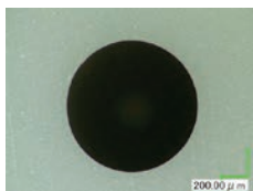
100th drilled hole No edge chipping
