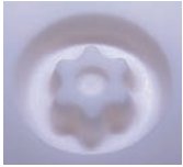
Alumina Al_2O_3
