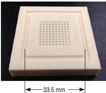
100th drilled hole No edge chipping
