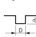
Slotting
